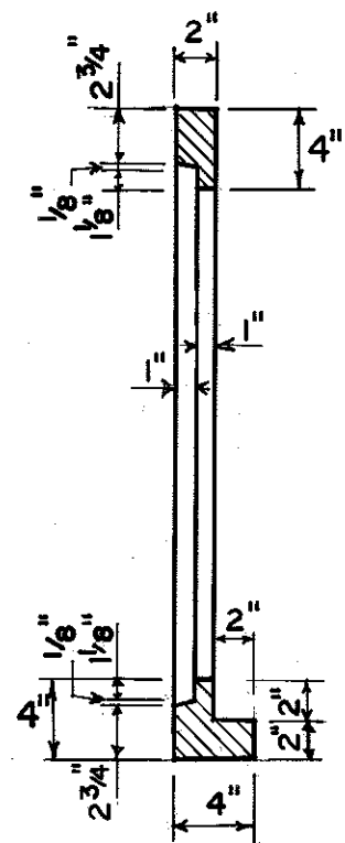
SECTION B-B
