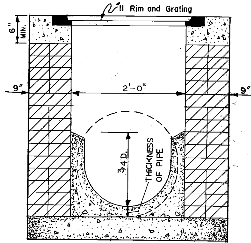
CROSS SECTION
