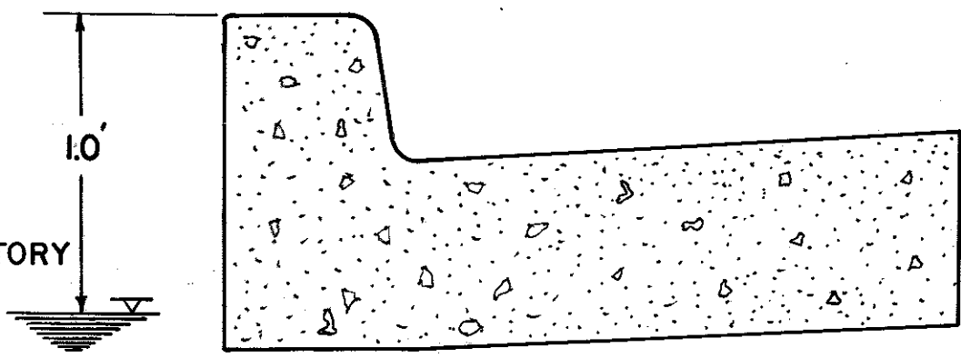
TYPICAL CURB & GUTTER
